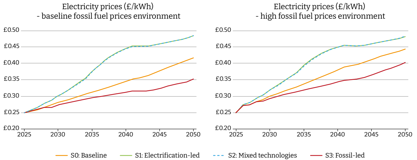
Figure 13: Electricity price trajectory
